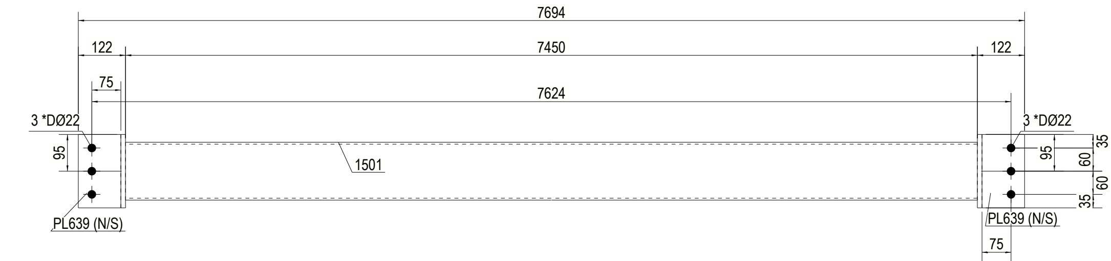
FRONT VIEW
